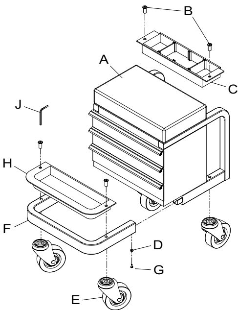
Figure 2 - 92450 Parts Breakdown
