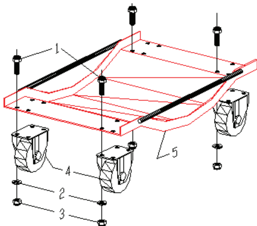
Fig. 3 - Assembly Illustration
