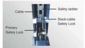
Double safety locks provide additional safety.
