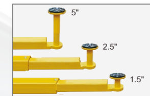
Standard drop-in adaptors 1.5", 2.5" & 5" extension high adaptors to fit different trucks and lifting height.
