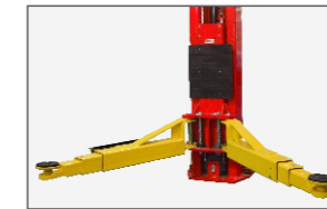
Three-stages Arms The OH-12 with 4 three-stages arms allowing to lift the trucks from short to long wheel base.
